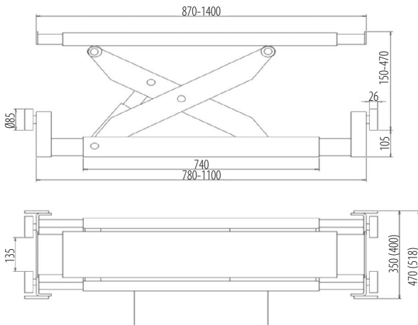
XT200P axis hoist 2T with hydraulic pump supplied pneumatically
