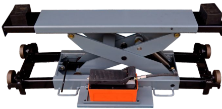
XT200H axis hoist 2T with manual hydraulic pump
